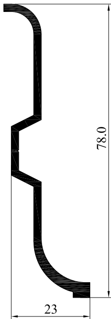
5777-20 0.572 Kg/m
