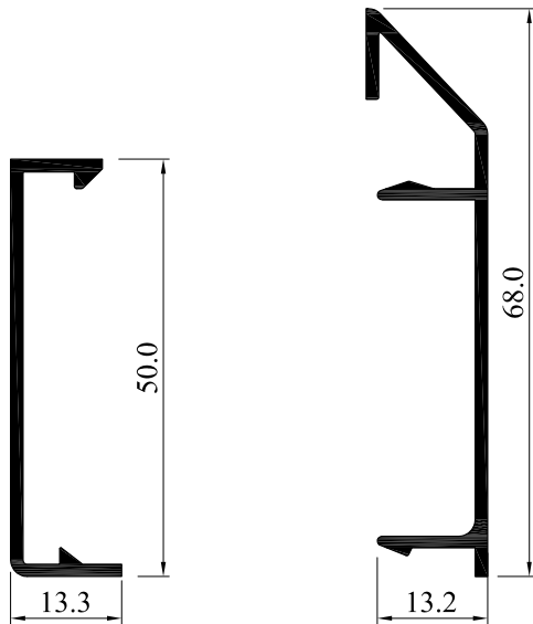
9606 0.304 Kg/m
