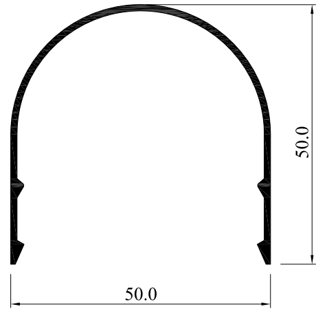
5306-12 0.431 Kg/m
