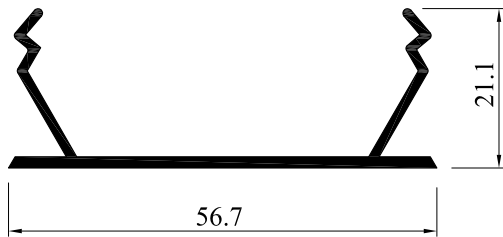
5307-15 0.378 Kg/m
