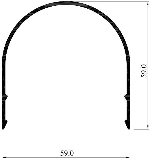
5308-15 0.629 Kg/m
