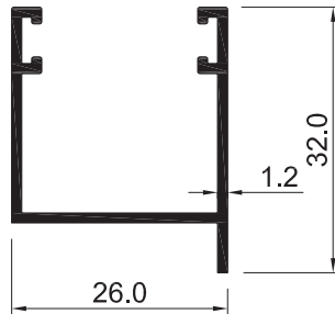
5507-12 0.307 kg/m
