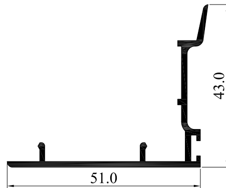
3154-15 0.452 Kg/m
