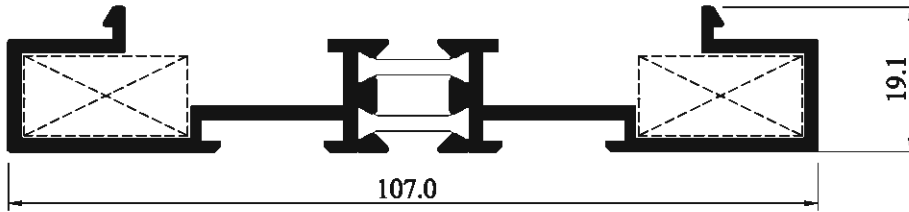
3211-16 Sabit Kasa ( Sabit Cam Kasa )
